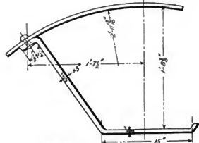
Fig. 264. Dry Pipe Hanger.
